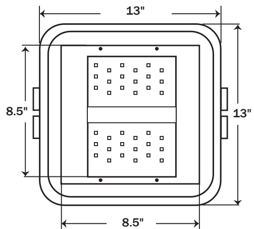
Scottsdale™* Low-Profile Adapter is approx. 1" deep
